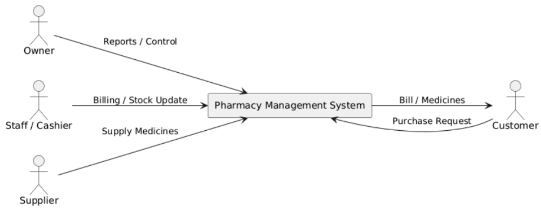
Figure 02: Context Diagram
